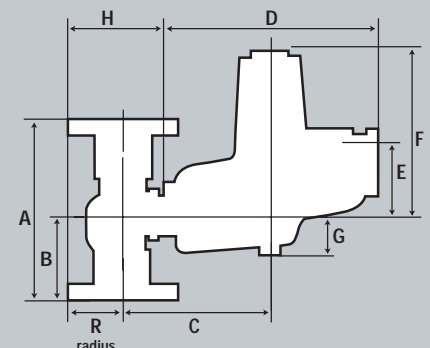
Flanged Valve Body
