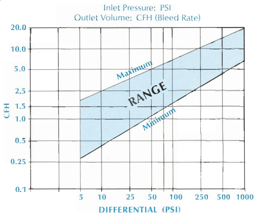
FLOW INHIBITOR BY-PASS RATE FOR VARIOUS INLET PRESSURES
